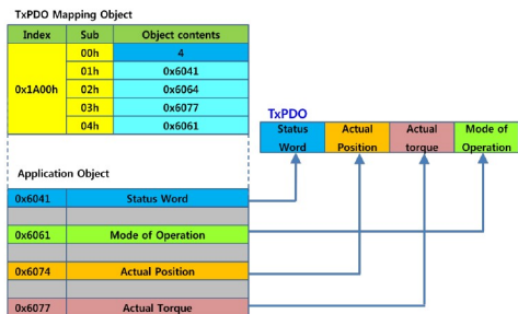
[1st TxPDO 맵핑 예]
